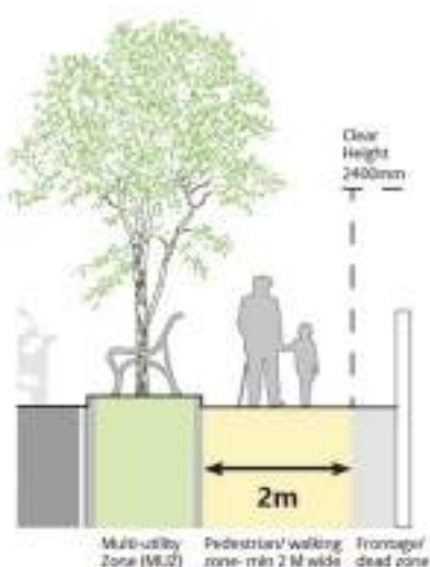
Figure 25. Typical footpath
