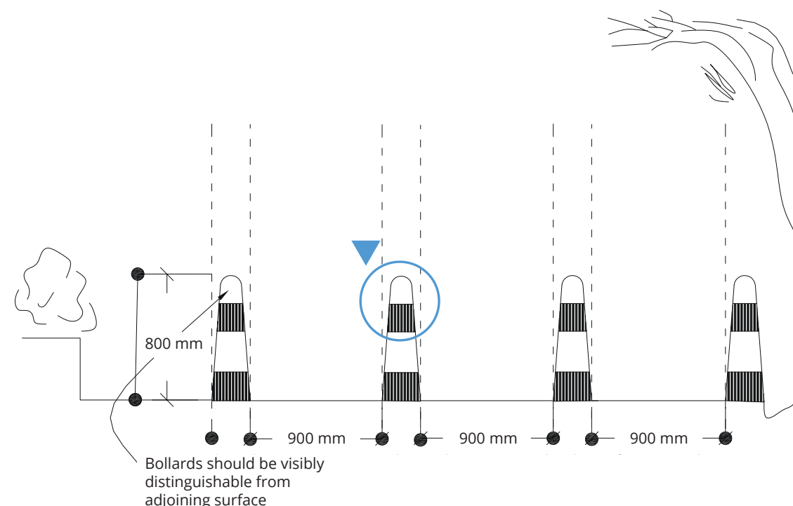
Figure 26. Spacing of bollards
